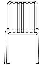
CHAIR W47 x D56 x H80 cm Seat height 45 cm, Seat depth 41 cm Stackable 8 pcs.
